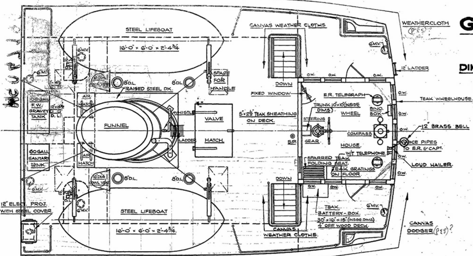
BOAT DECK & BRIDGE DECK.
