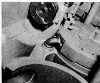
Upper Water Jumper from Cylinder Head
