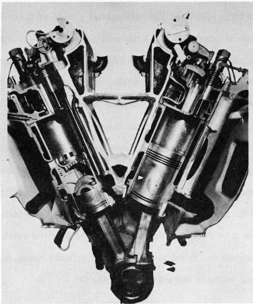
(Fig. 48) Section-Original 567 Design
